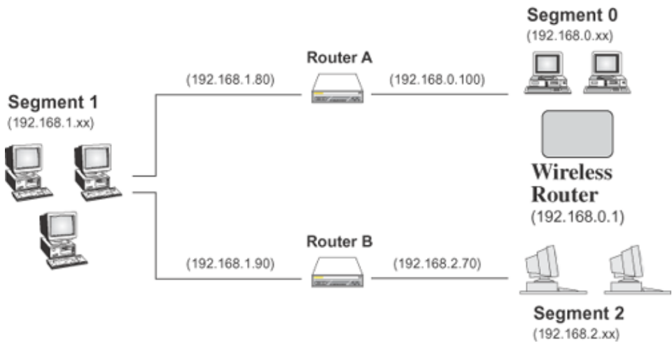
Routing Example
