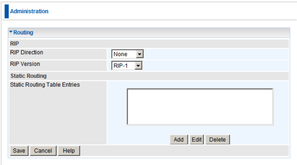
Routing Screen
